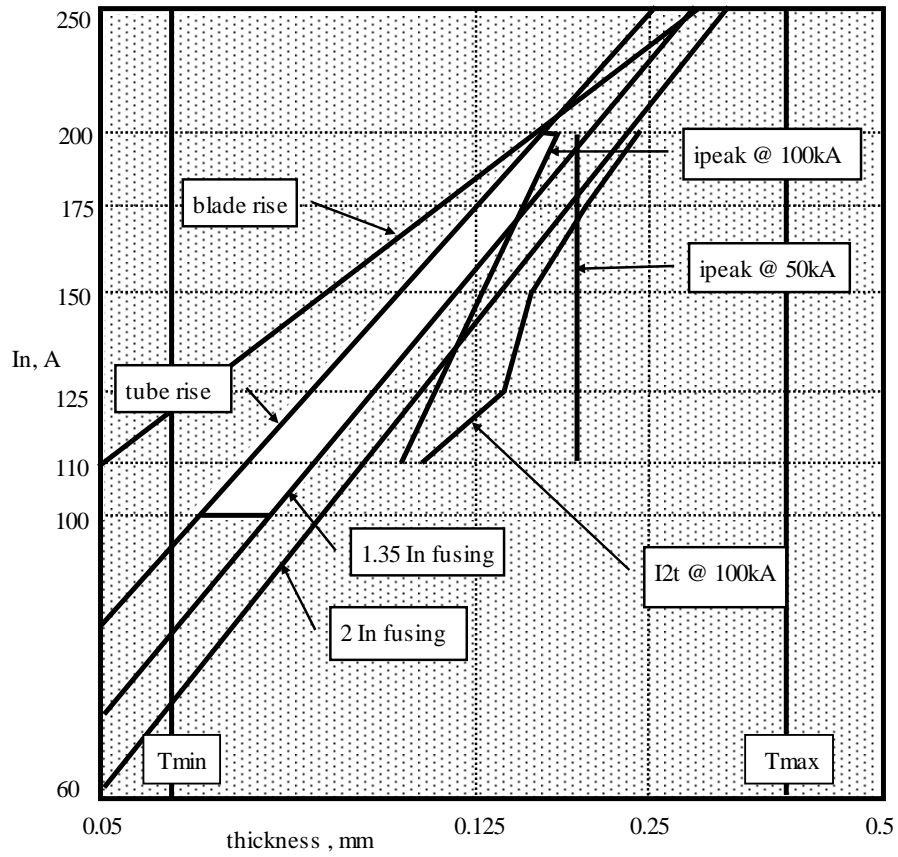
Fig. 9: Example showing all constraints and feasible solution space for a fast-acting class J fuse.
