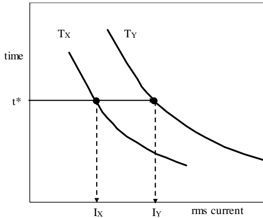
Fig. 3: Time-current test data in the vicinity of a specified fusing (or nonfusing) time for two different element thicknesses.
