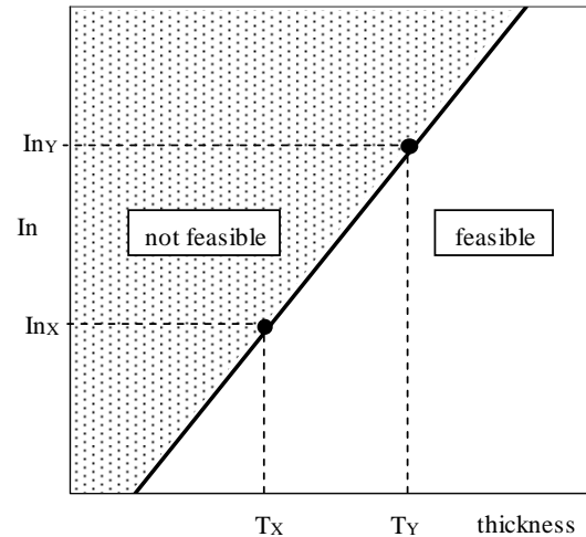
Fig. 2: Maximum possible current rating, based on a temperature-rise test limit.
