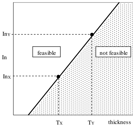
Fig. 4: Minimum current rating to meet a specified fusing requirement.
