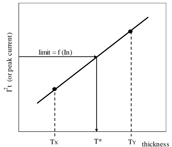
Fig. 6: I^2t or i_{peak} test data for two different fuse element thicknesses at a specified prospective current.
