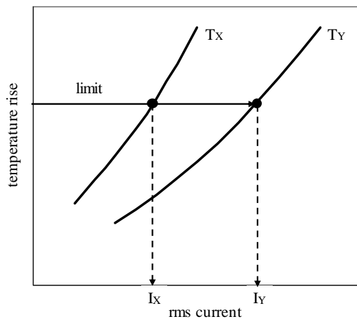
Fig. 1: Temperature rise versus test current for two different fuse element thicknesses.
