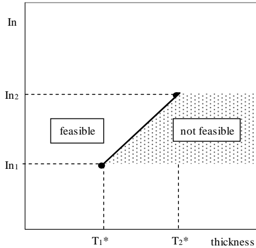
Fig. 7: Minimum possible current rating, based on I^2t or i_{peak} requirements.
