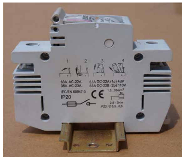
Fig. 3: Switch-disconnector-fuse type STV D02-1.
